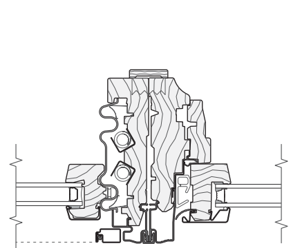
VERTICAL JOINING MULLION VENT / FIXED
