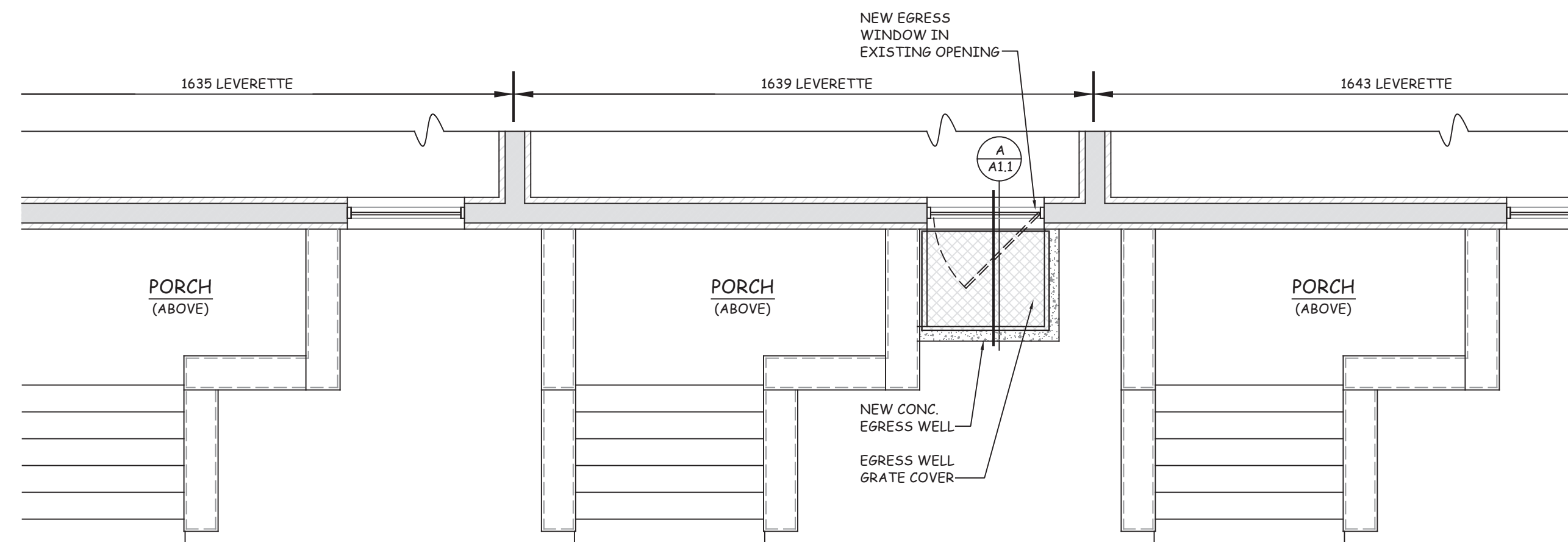
PROPOSED LOWER LEVEL PLAN SCALE: 1/4" = 1'-0"
