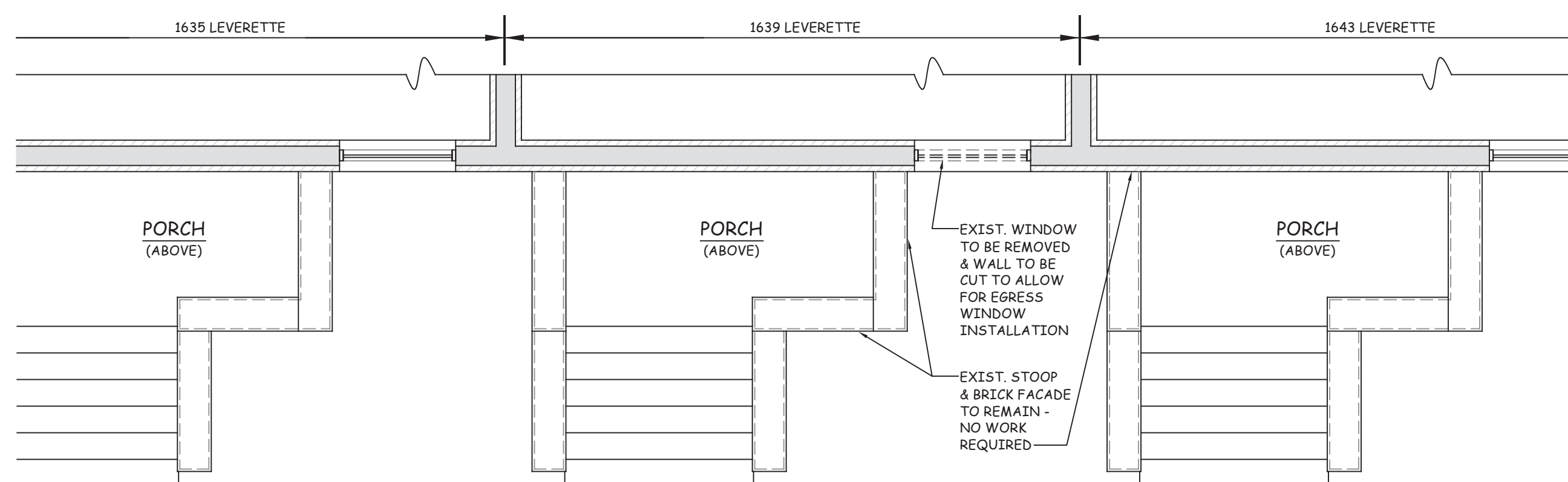
EXISTING LOWER LEVEL PLAN SCALE: 1/4" = 1'-0"
