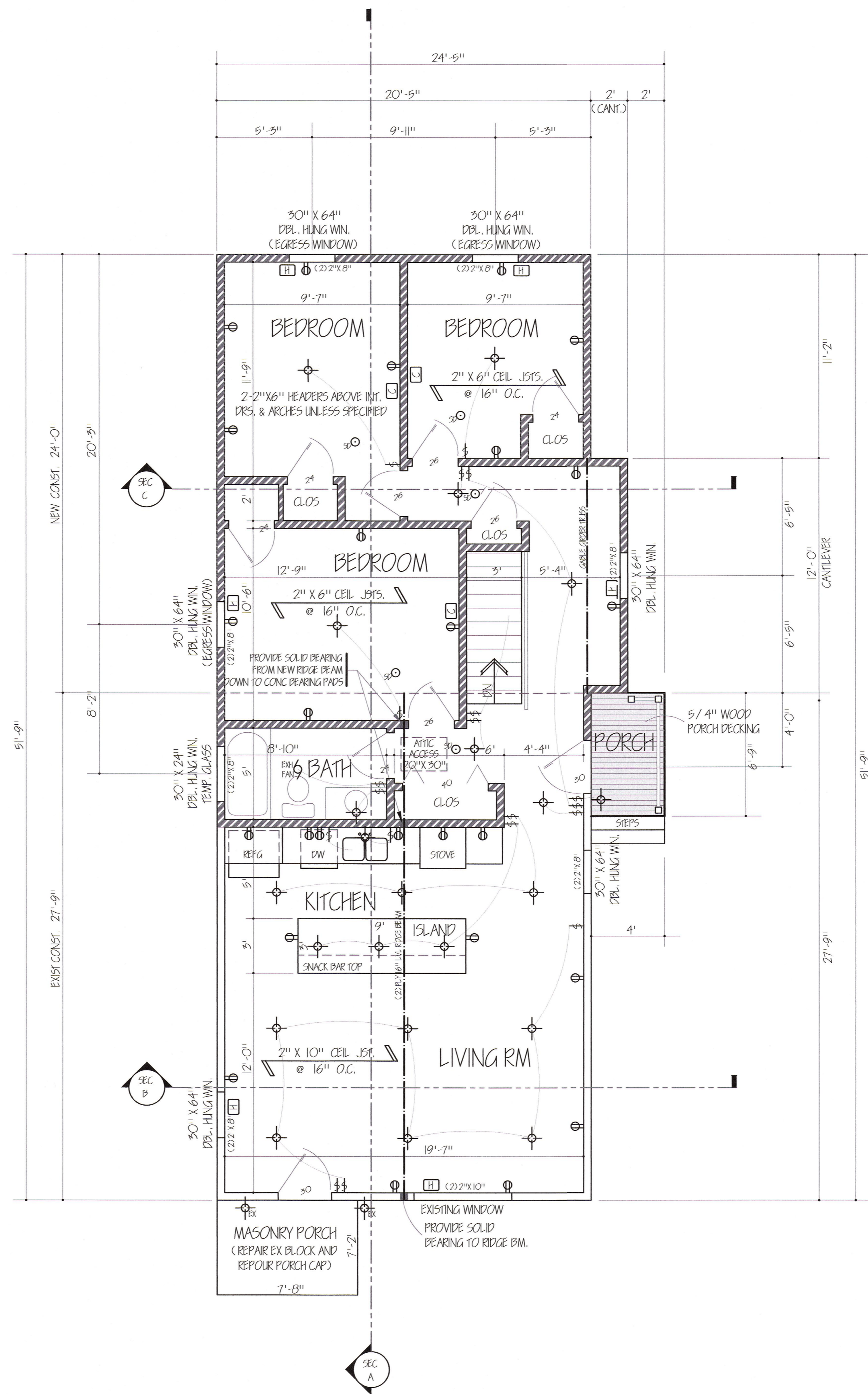
PROPOSED FLOOR PLAN
