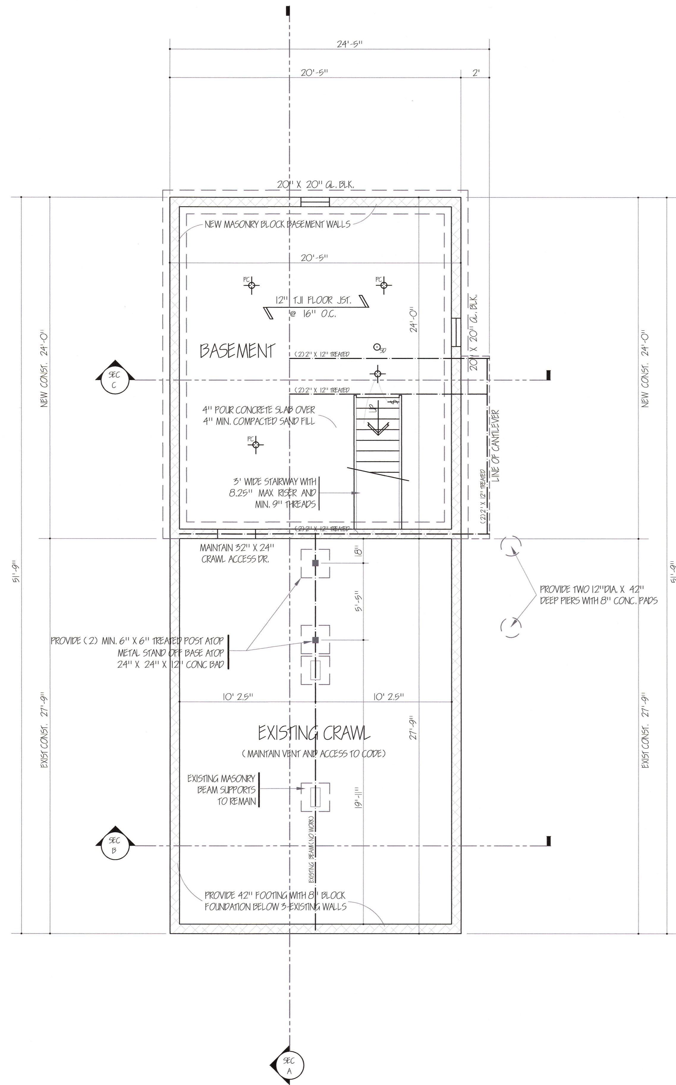
FOUNDATION PLAN
