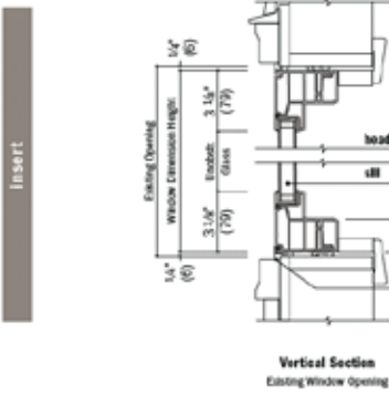
Picture, Single Transom and Specialty Window Details - Replacement (continued) Scale 1 1/2" (38) = 1'-0" (305) - 1:8
