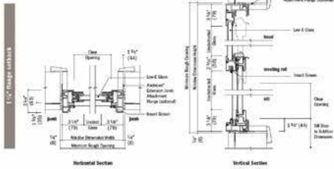
Single-Hung Window Details - New Construction Scale 1 1/2" (38) = 1'-0" (205) - 1:8
