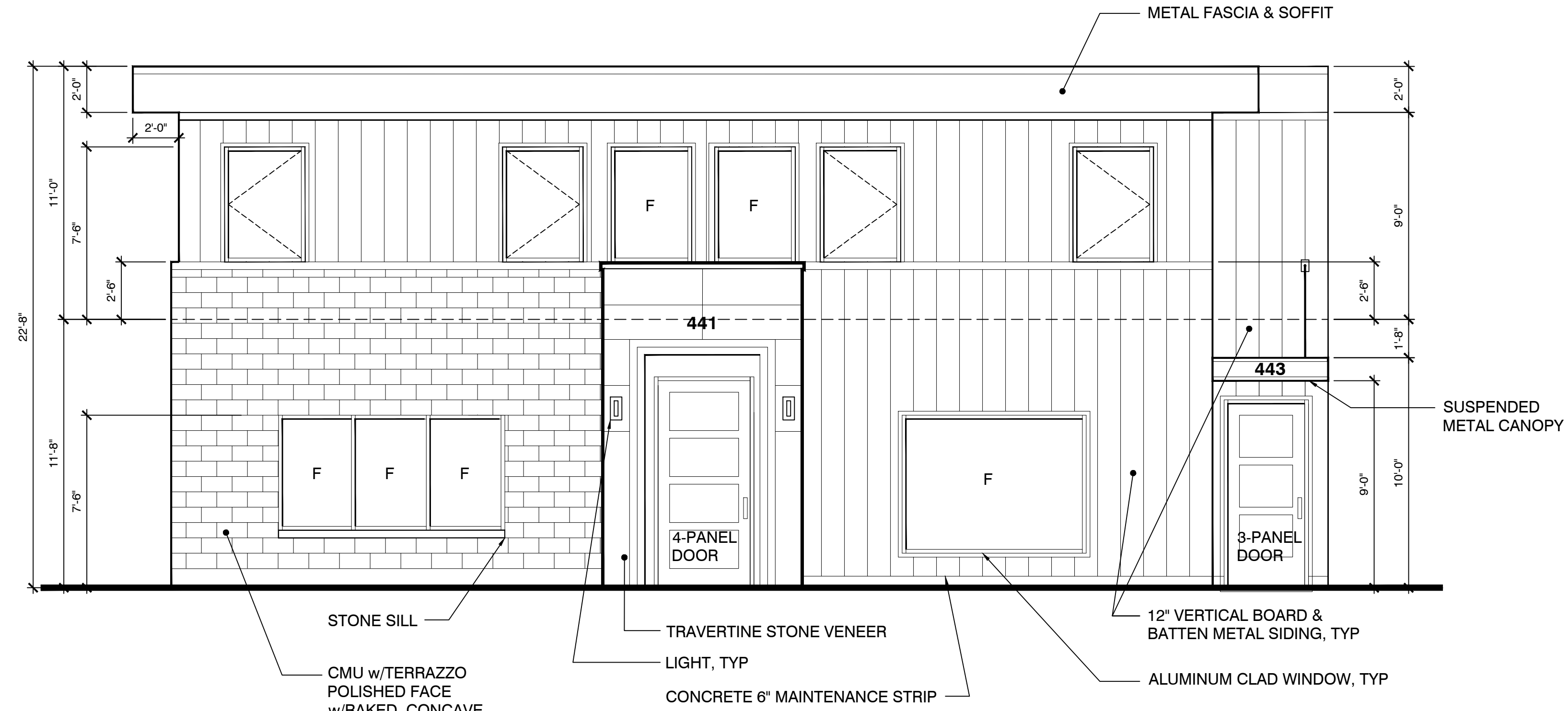
1 BUILDING ELEVATION - NORTH SCALE: 1/4" = 1'-0"
