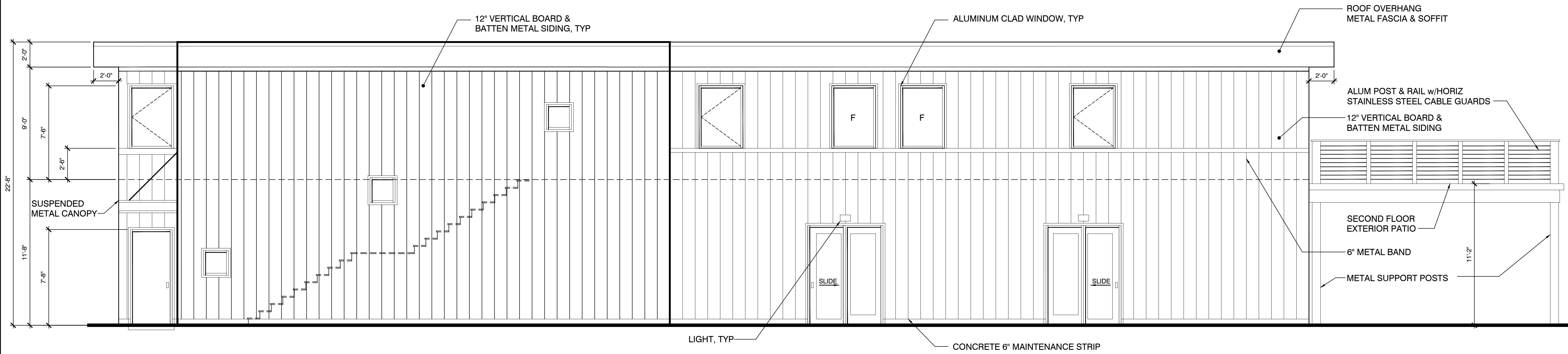
2 BUILDING ELEVATION - WEST SCALE: 1/4" = 1'-0"
