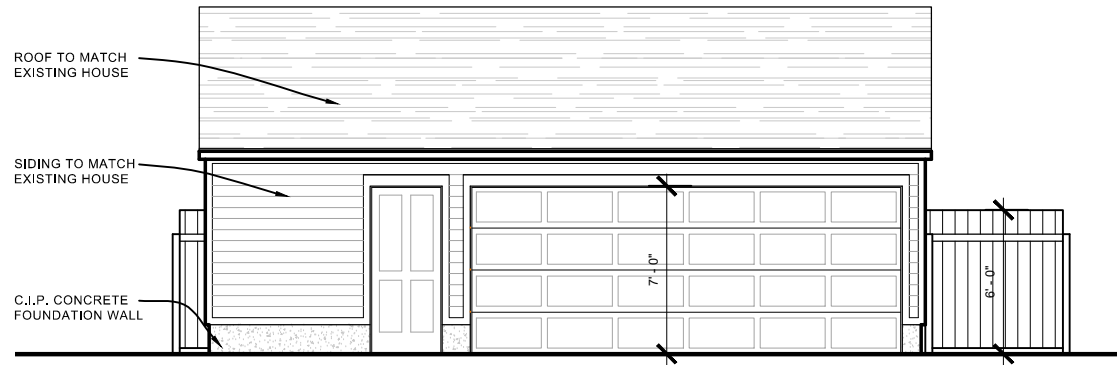
2 WEST ELEVATION
