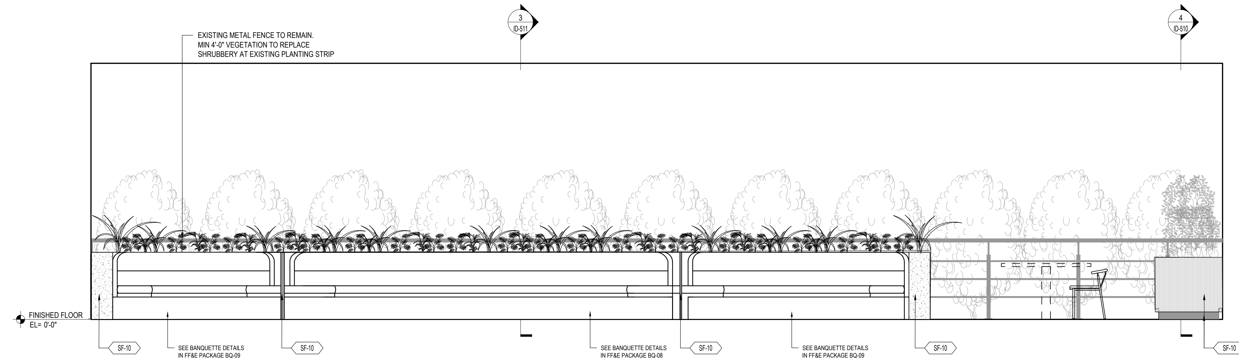
5 INTERIOR ELEVATION - PATIO SCALE: 3/8"=1'-0"
