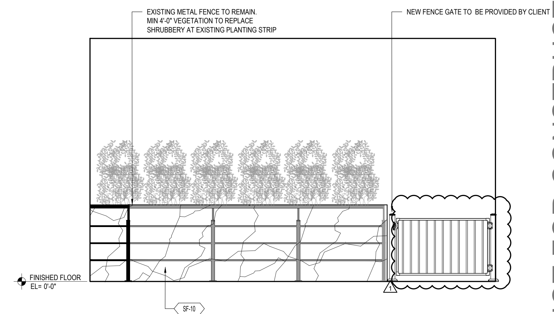
3 INTERIOR ELEVATION - PATIO SCALE: 3/8"=1'-0"
