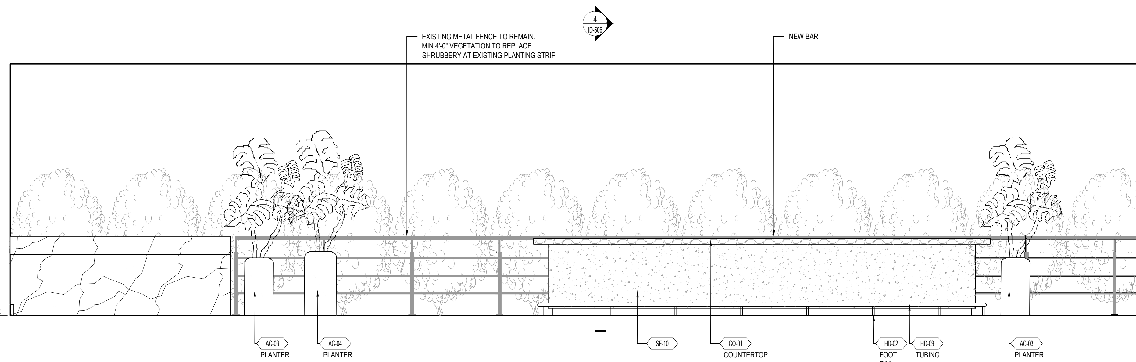
2 INTERIOR ELEVATION - PATIO SCALE: 3/8"=1'-0"
