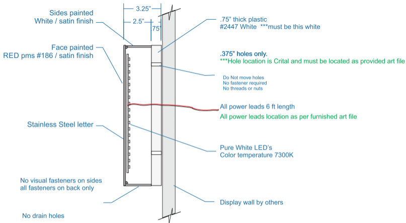
Section Detail
