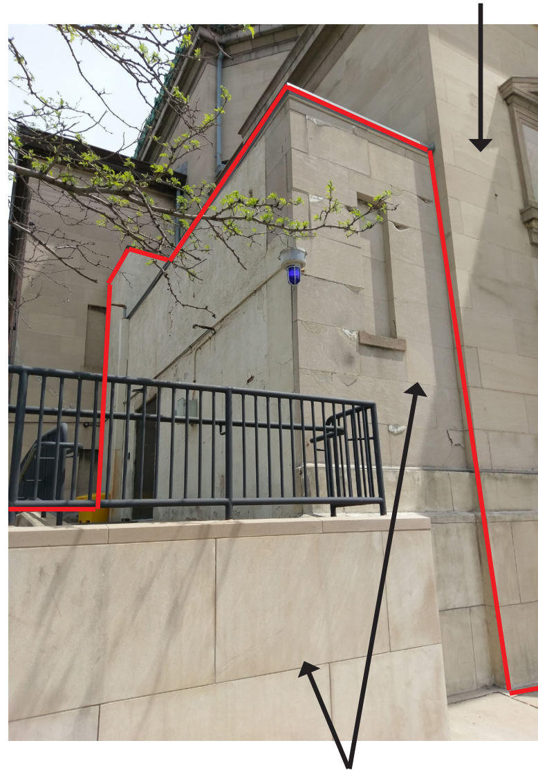
ACCESS RAMP TO BE DEMOLISHED. LATER ADDITION TO BE INTEGRATED INTO NEW ENTRY
