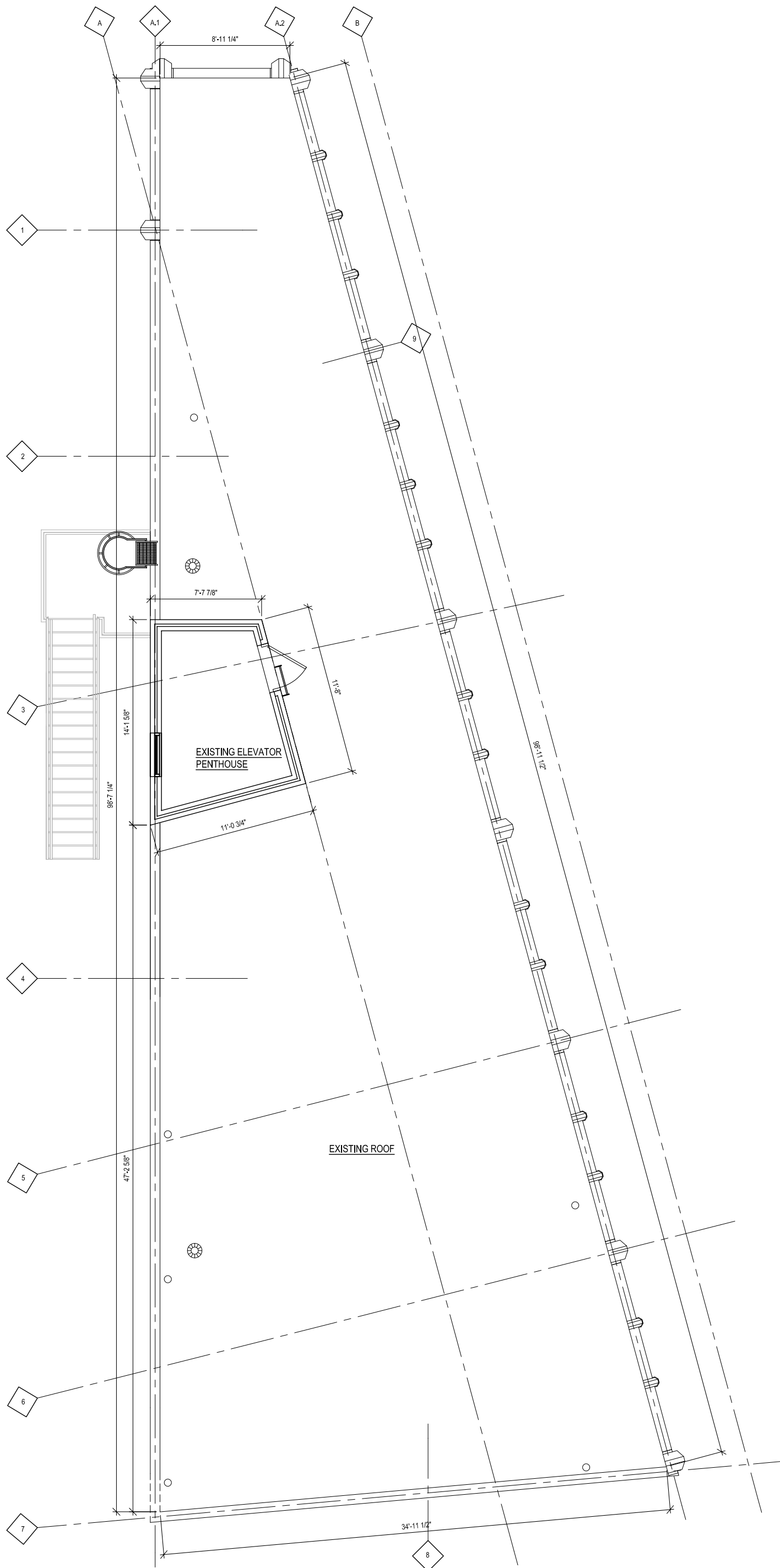
1 EXISTING ROOF PLAN AD102 1/4" = 1'-0"
