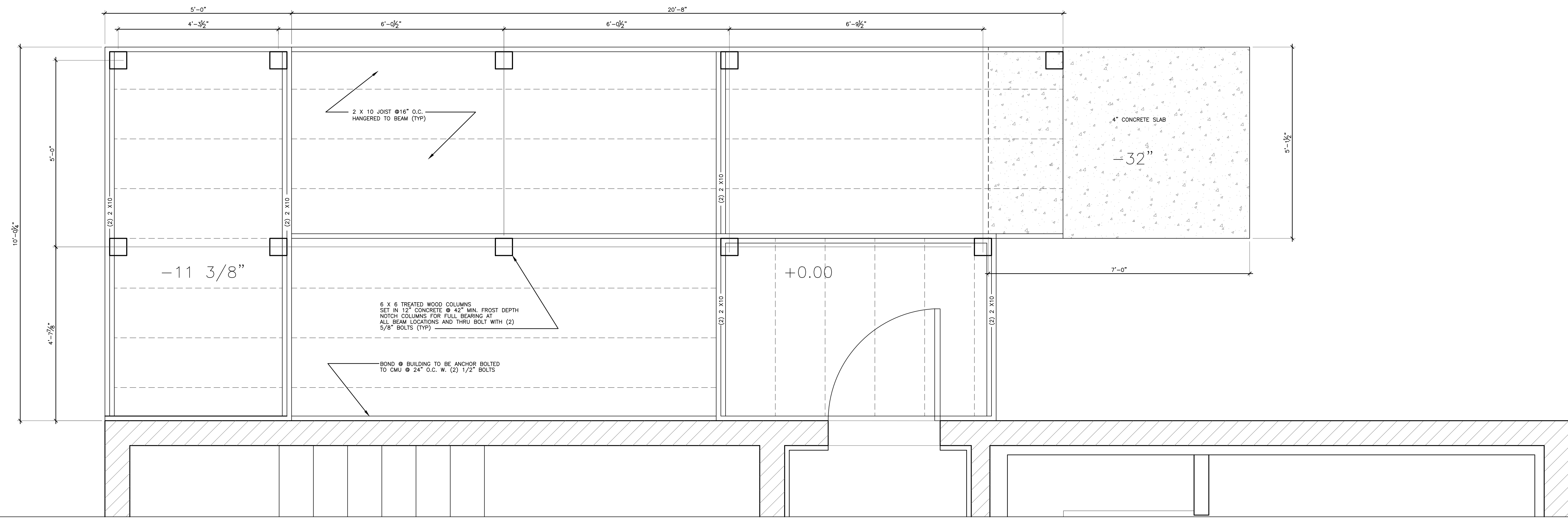
NEW ADA EGRESS RAMP FRAMING DETAIL
