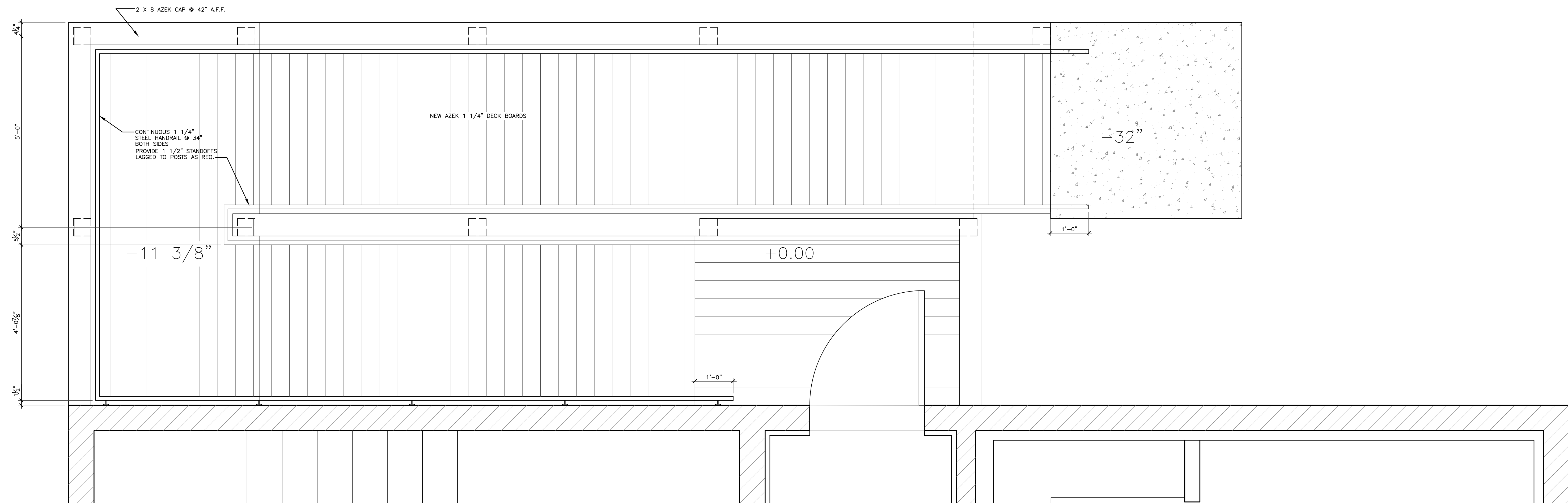
NEW ADA EGRESS RAMP DETAIL
