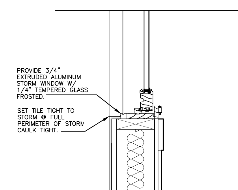
SHOWER WINDOW DETAIL 1/2" = 1'-0" UNITS 101, 201, 202
