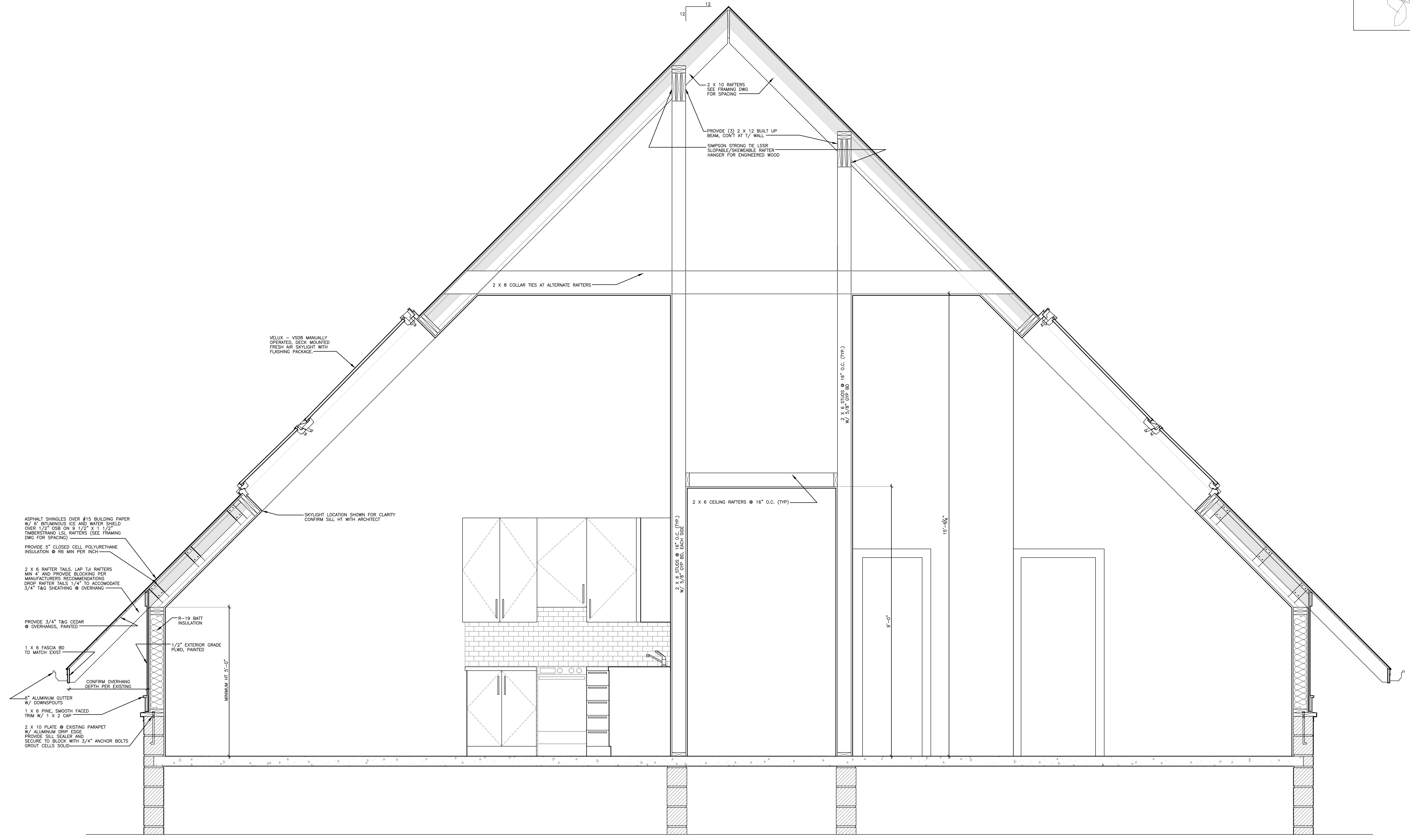
SECTION AT 3RD FLOOR ADDITION 3/4" = 1'-0"
