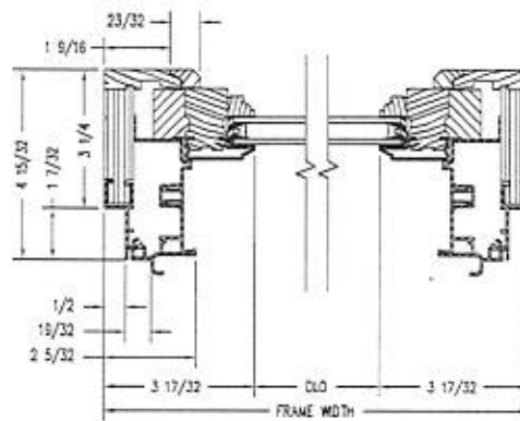
Horizontal Section
