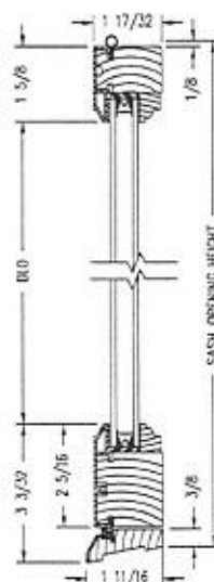
Vertical Section
