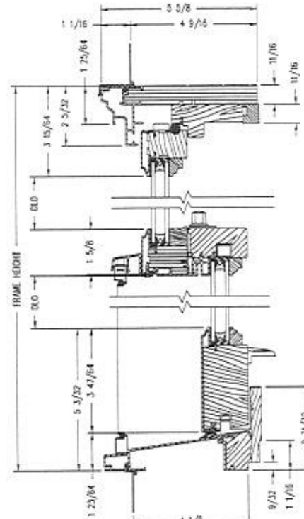
Vertical Section
