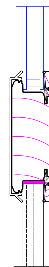
9 4 INTERMEDIATE RAIL SCALE: 6" = 1'-0"
