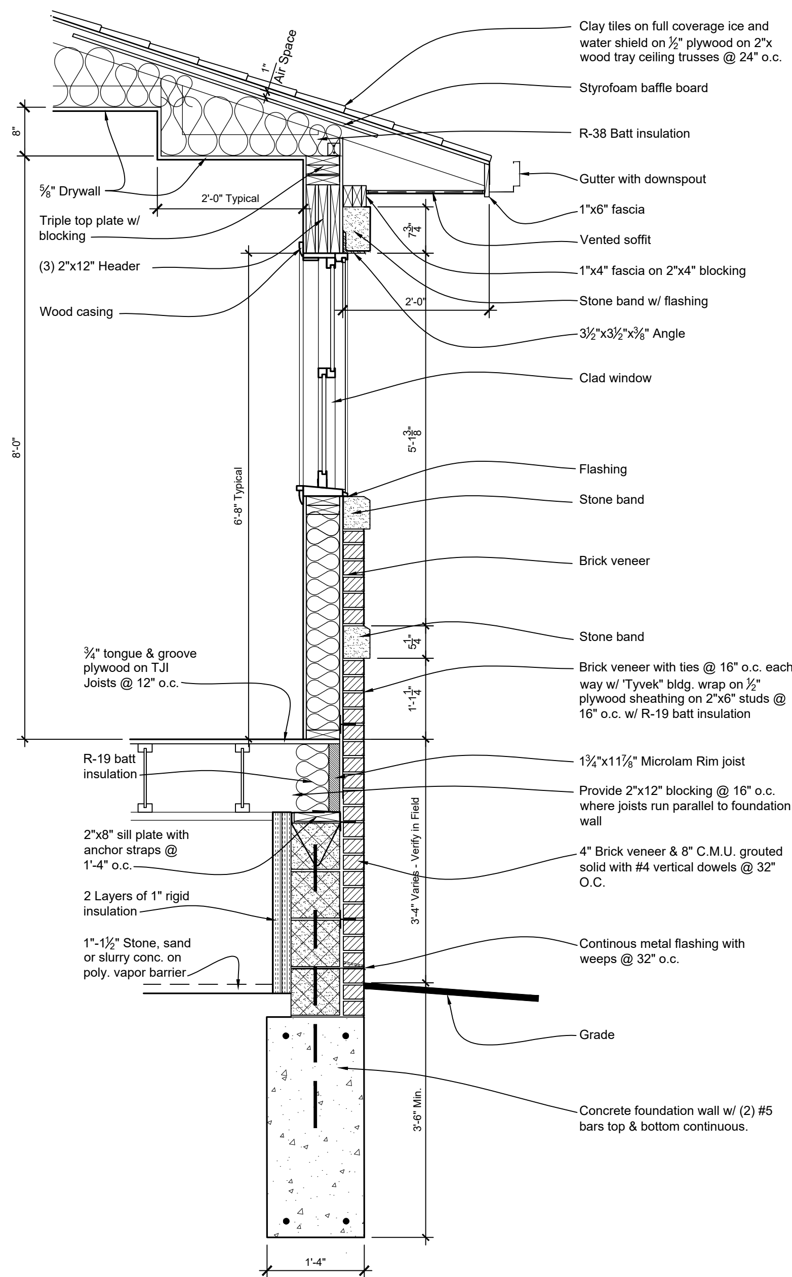
1 A-01 Typical Section Scale: 3/4"=1'-0"
