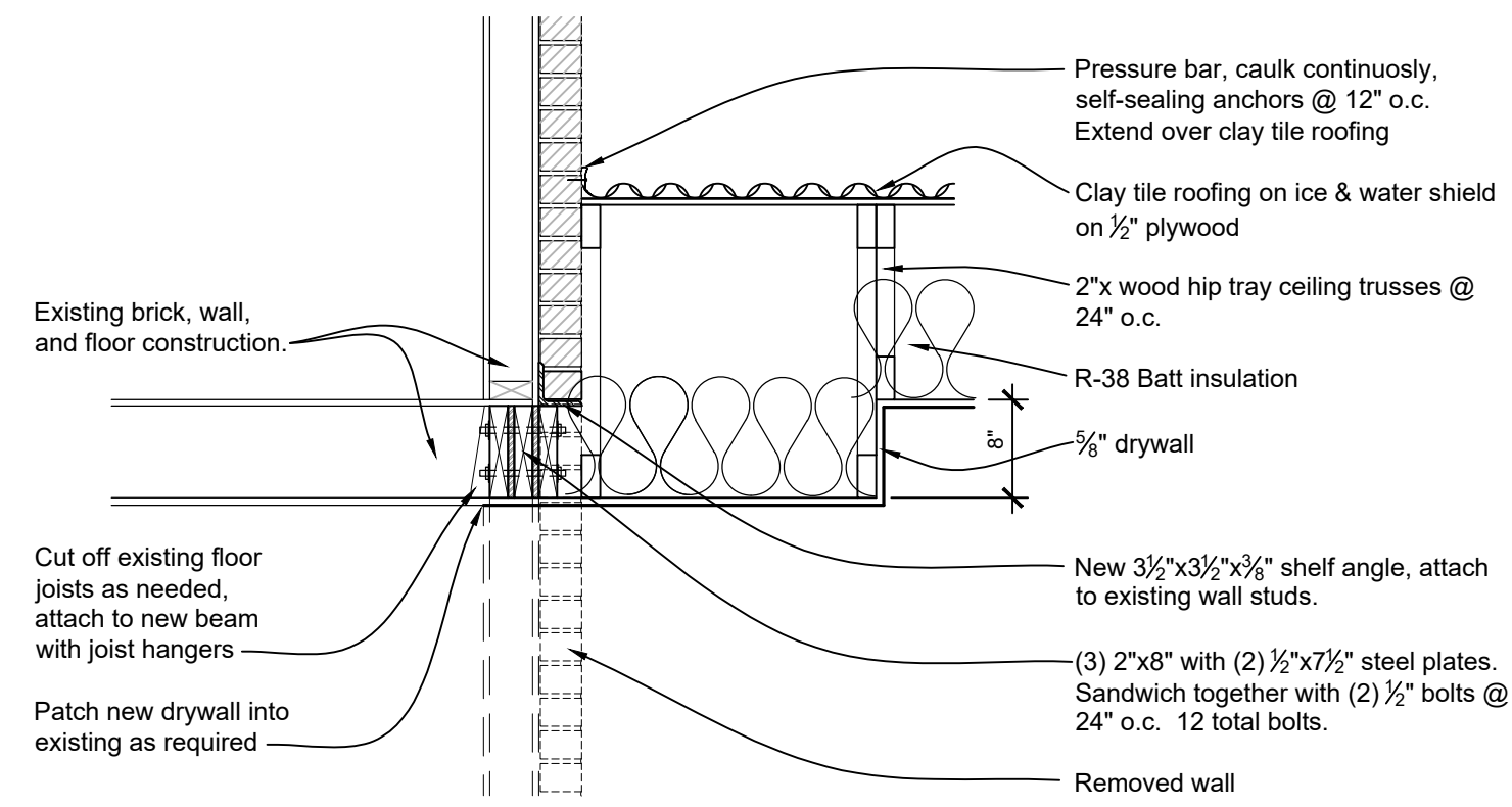
2 A-01 Beam Detail Scale: 1/2"=1'-0"
