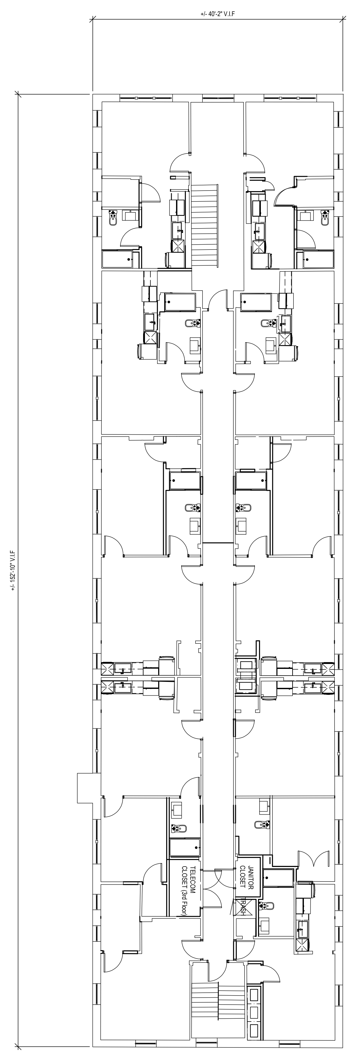
489 HENRY FLOOR PLAN 2-4 1 1A102 1/8" = 1'-0"
