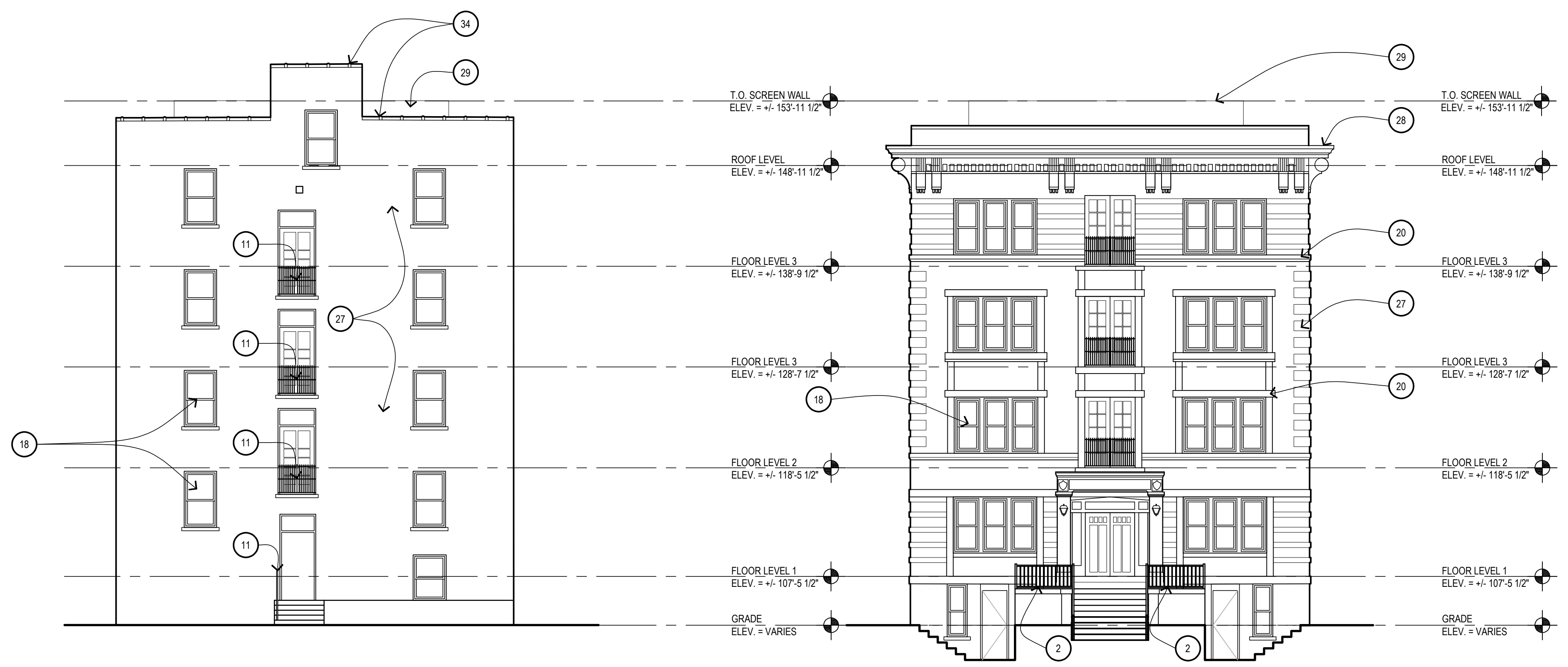
3 1A401 489 HENRY SOUTH EXTERIOR ELEVATION 1/8" = 1'-0"
