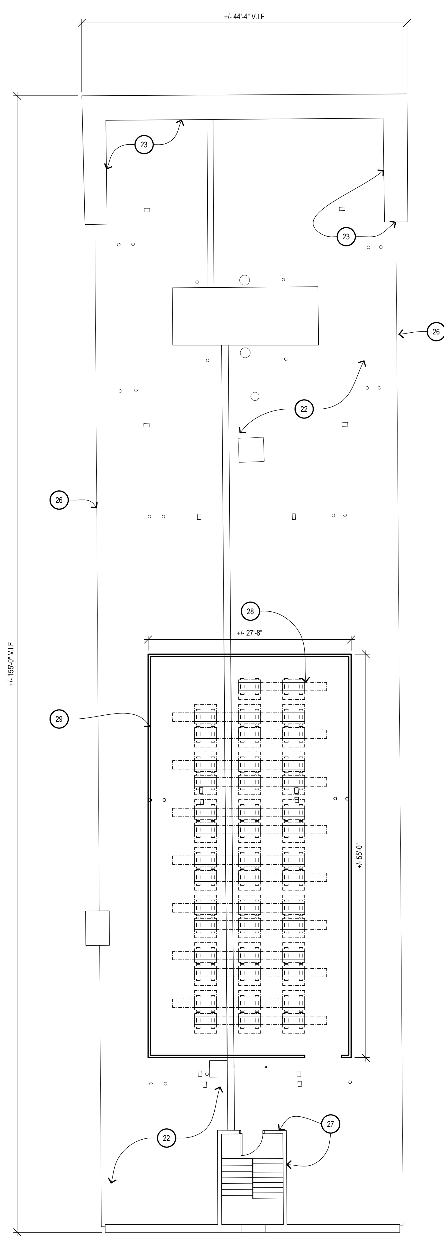
489 HENRY ROOF 2 1A102 1/8" = 1'-0"
