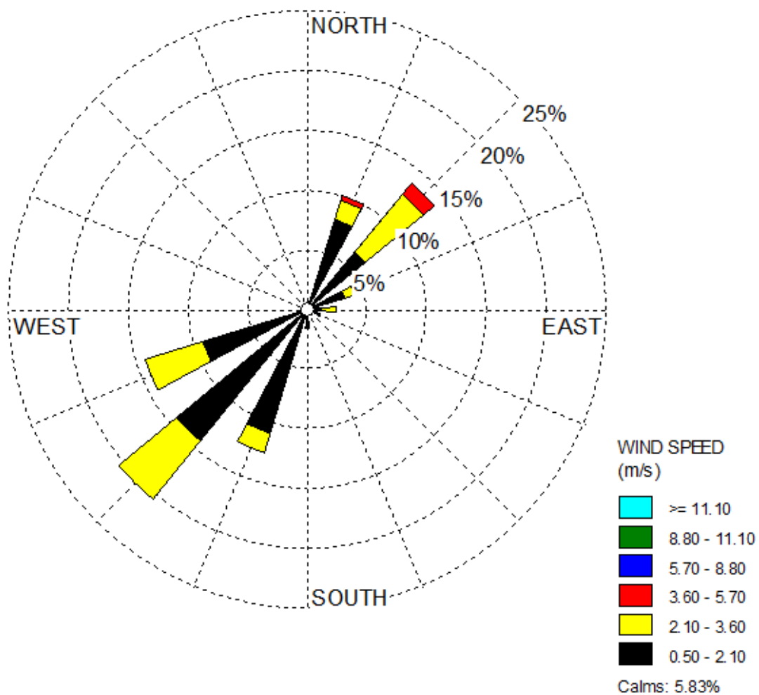
Figure 2-A – Wind Rose From 1479 Monitor
