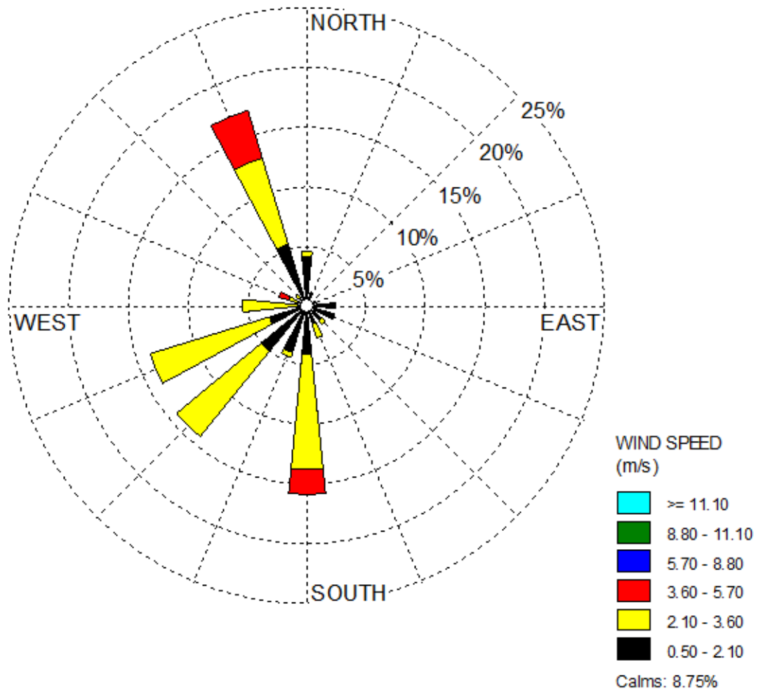
Figure 2-B – Wind Rose From 1480 Monitor
